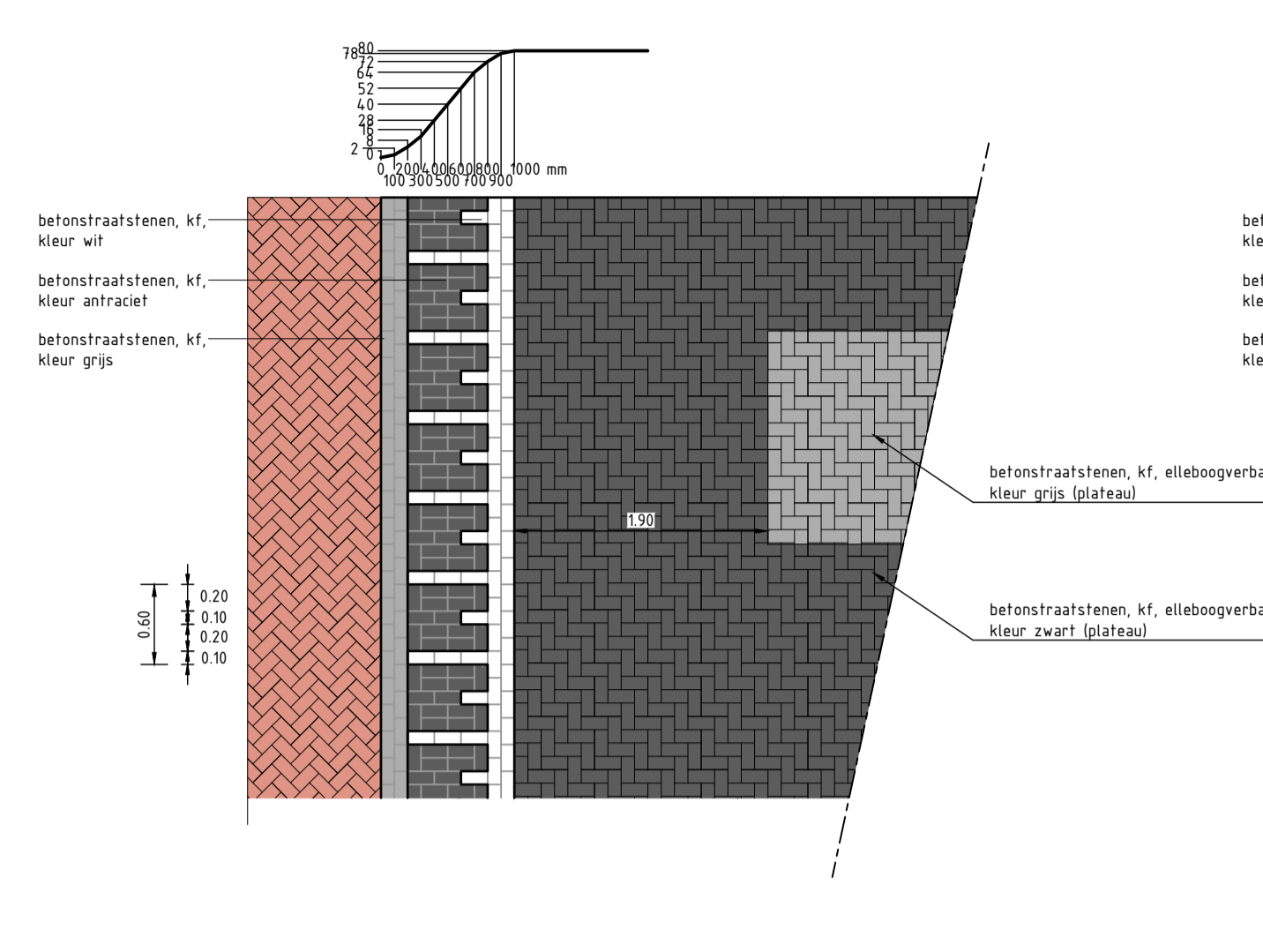
Detail, plateauoprit, 30km/u Schaal 1:50
